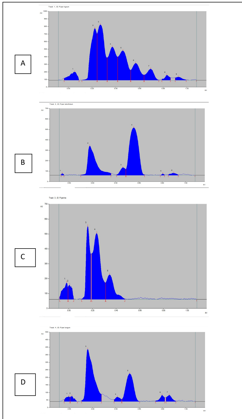
Figure 5: HPTLC fingerprint patterns of 3 Piper species with the piperine standard A: P. nigrum , B: P. retrofractum , C: Piperine, D: P. longum
