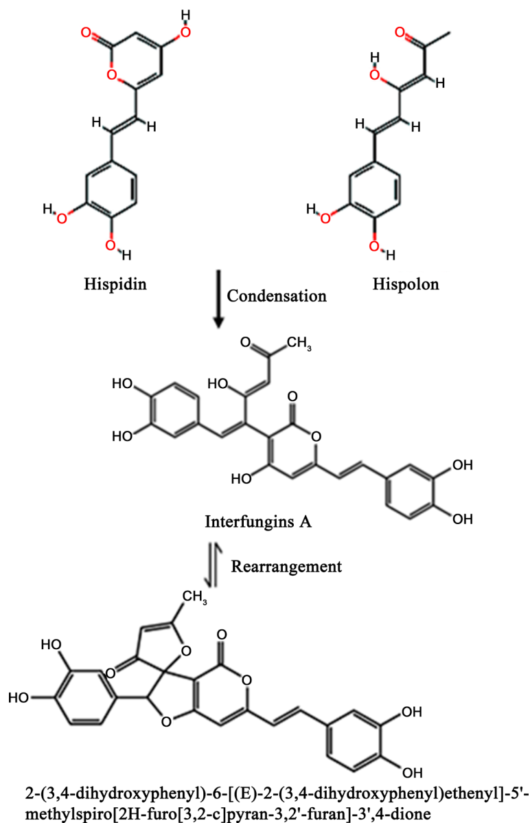
Figure 2. Biosynthetic pathway of 2-(3,4-dihydroxyphenyl)-6-[(E)-2-(3,4-dihydroxyphenyl)ethenyl]-5'-methylspiro[2H-furo[3,2-c]pyran-3,2'-furan]-3',4-dione via rearrangement of interfungins A, which is resulted from the condensation of hispidin and hispolon moieties.
