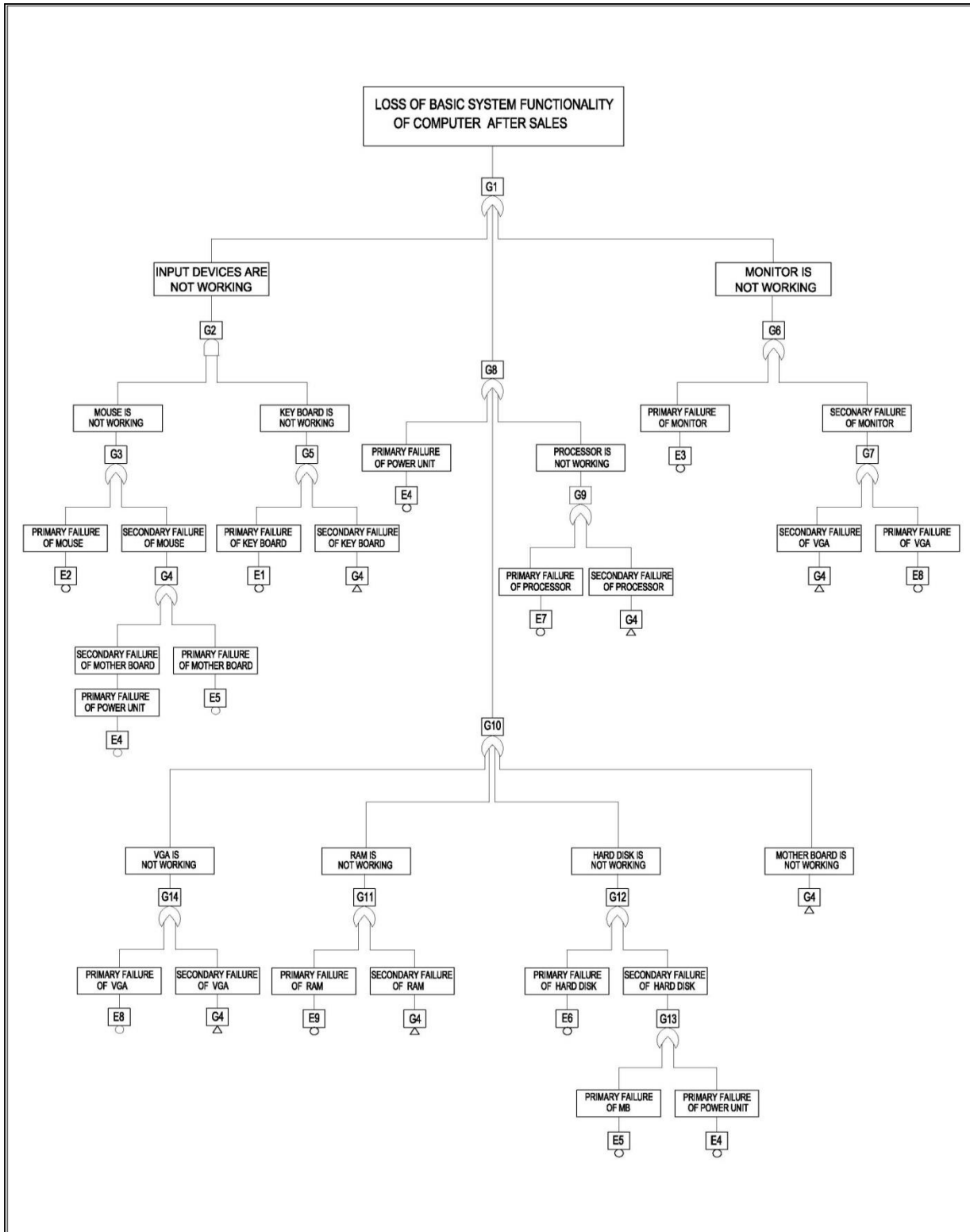
FIGURE 1 - FAULT TREE OF THE PERSONAL COMPUTER SYSTEM
